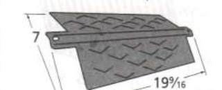
96411 porcelain steel
