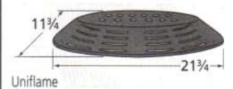
99351 porcelain steel
